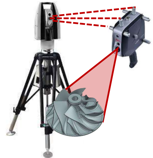
Laser tracker and scanner head
