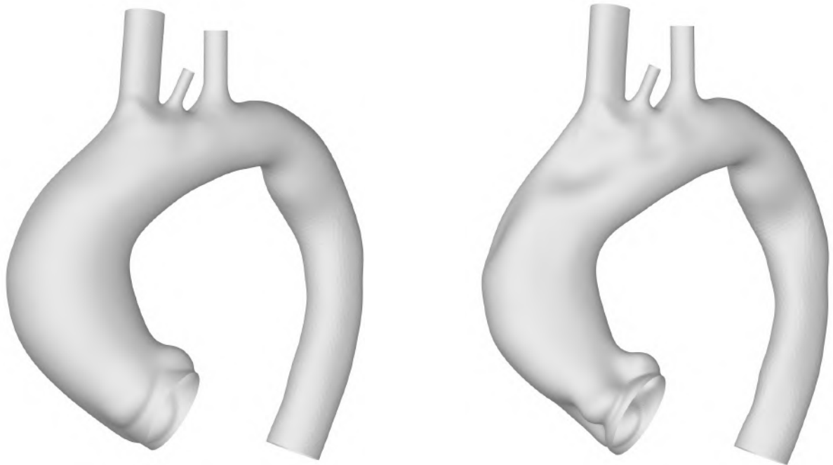
Figure 5.23: Reference configuration \mathbf{X}^* (left) and zero-pressure configuration \mathbf{X}_{\text{ZP}} (right).
